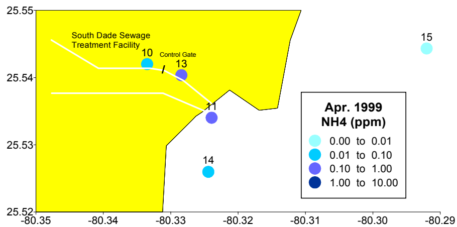
Figure 8. Map of \text{NH}_4^+ concentrations at landfill sites in Apr. 1999.
