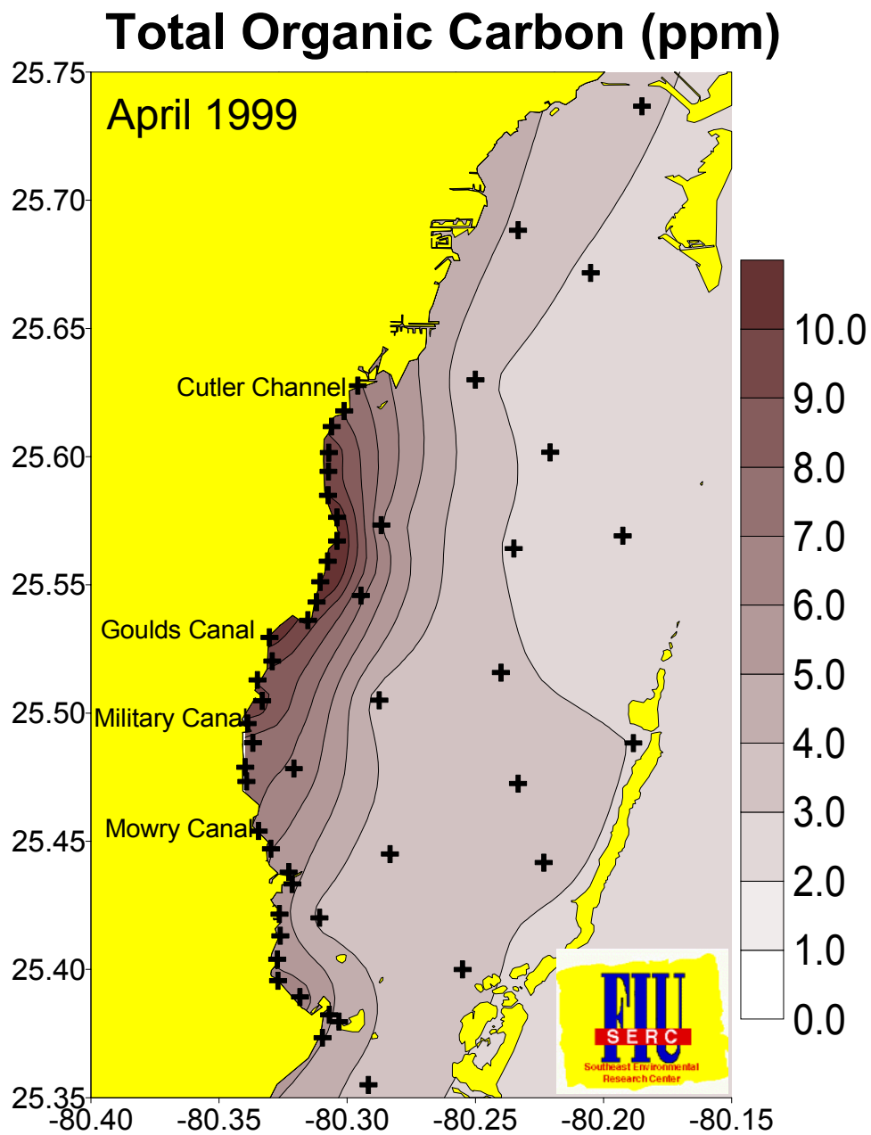
Figure 26. Total organic carbon data from combined Shoreline Ammonia Survey and April 1999 FIU Biscayne Bay water quality monitoring program. Note elevated inshore concentrations occurring from Cutler Canal to Mowry Canal.
