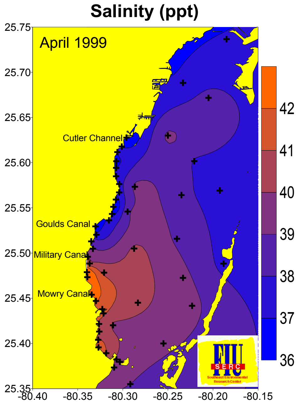
Figure 21. Salinity data from combined Shoreline Ammonia Survey and April 1999 FIU Biscayne Bay water quality monitoring program. Note hypersaline conditions in the south below Military Canal.
