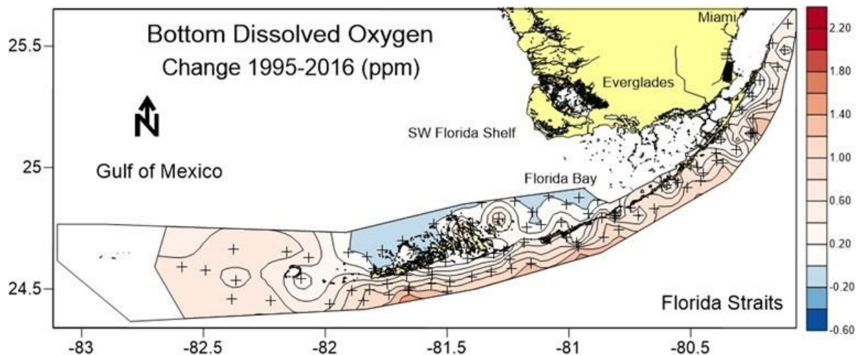
Figure iii. Total change in DO of bottom waters for 22 year period calculated from significant trends.
