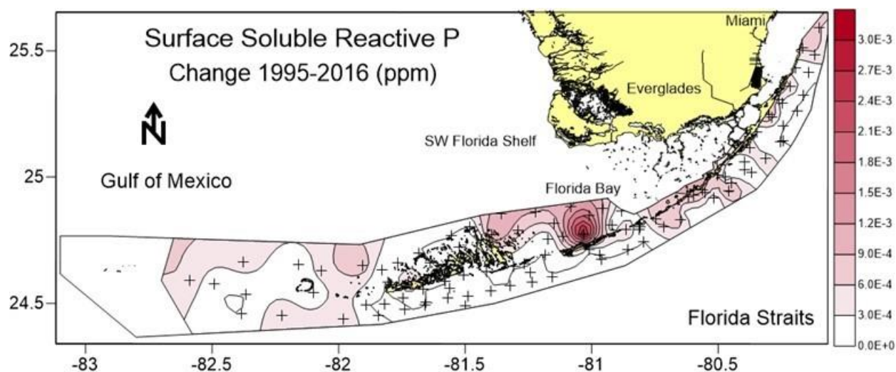
Figure vi. Total change in SRP in surface waters for 22 year period calculated from significant trends.
