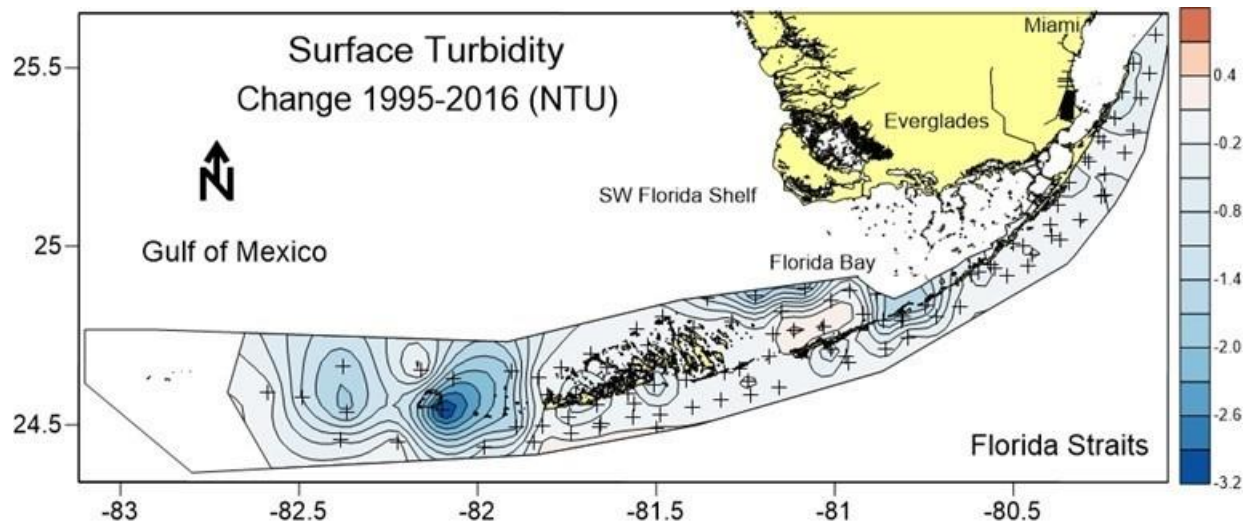
Figure iv. Total change in Turbidity in surface waters for 22 year period calculated from significant trends.
