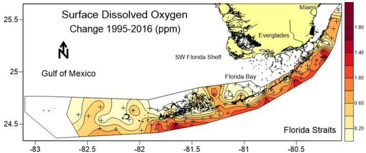
Figure ii. Total change in DO of surface waters for 22 year period calculated from significant trends.
