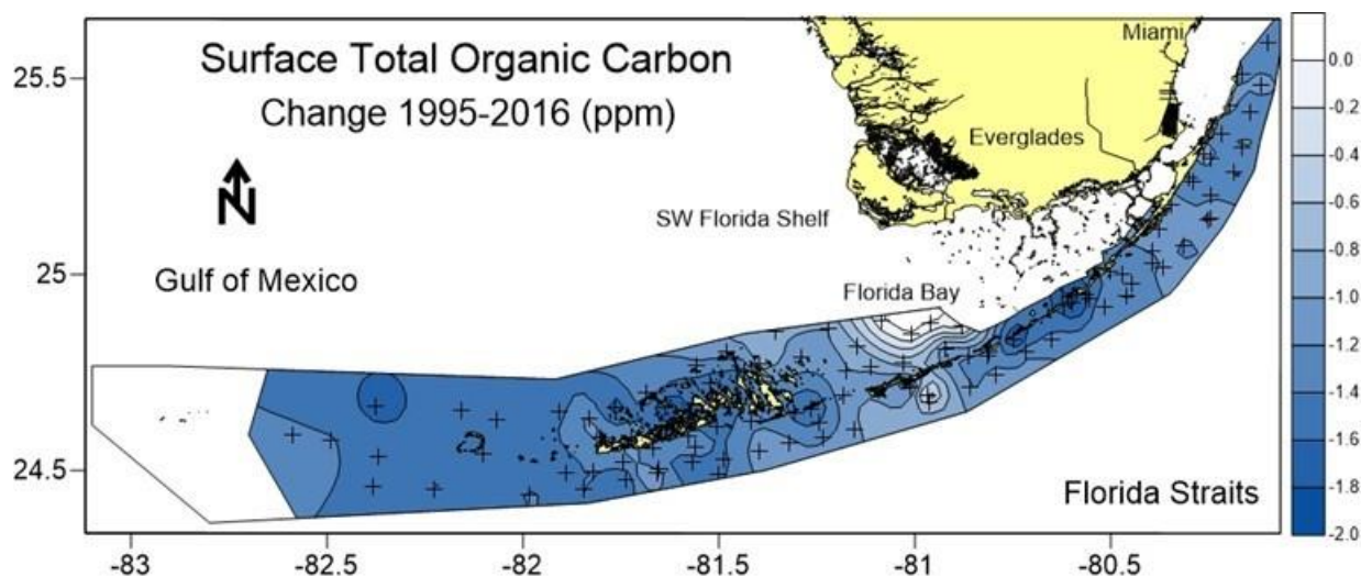
Figure vii. Total change in TOC in surface waters for 22 year period calculated from significant trends.
