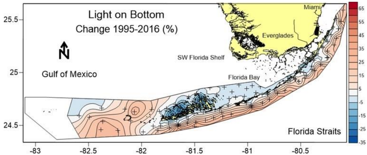
Figure v. Total change in bottom I_o for 22 year period calculated from significant trends.
