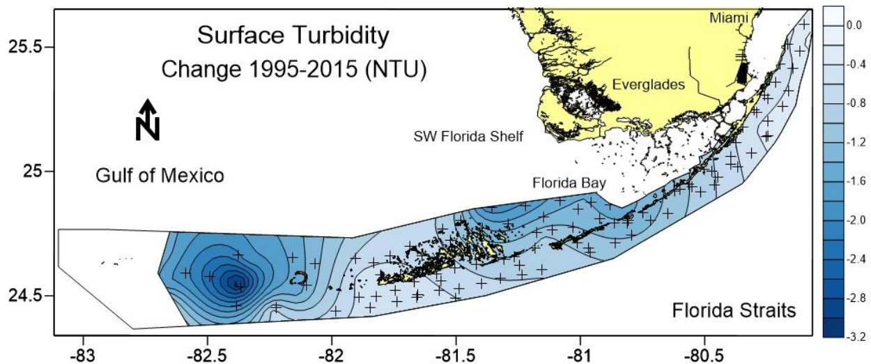
Figure iv. Total change in Turbidity in surface waters for 20 year period calculated from significant trends.
