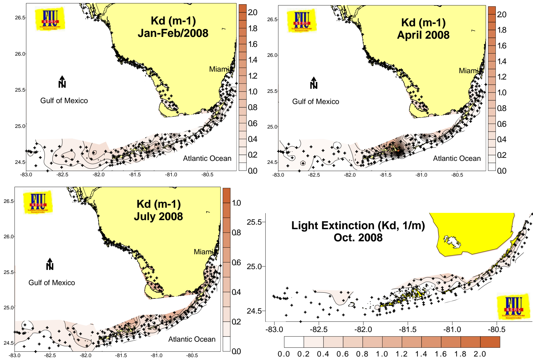
Figure 34. Distributions of Light extinction across the region during 2008.
