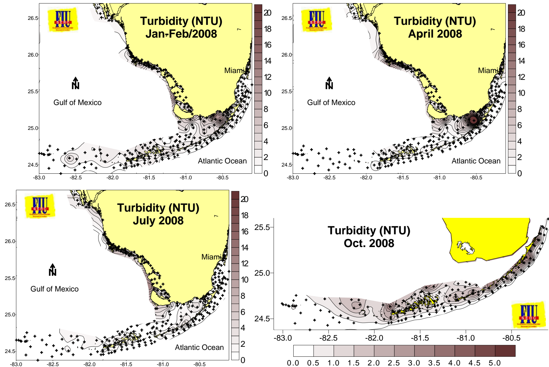
Figure 33. Distributions of turbidity across the region during 2008.
