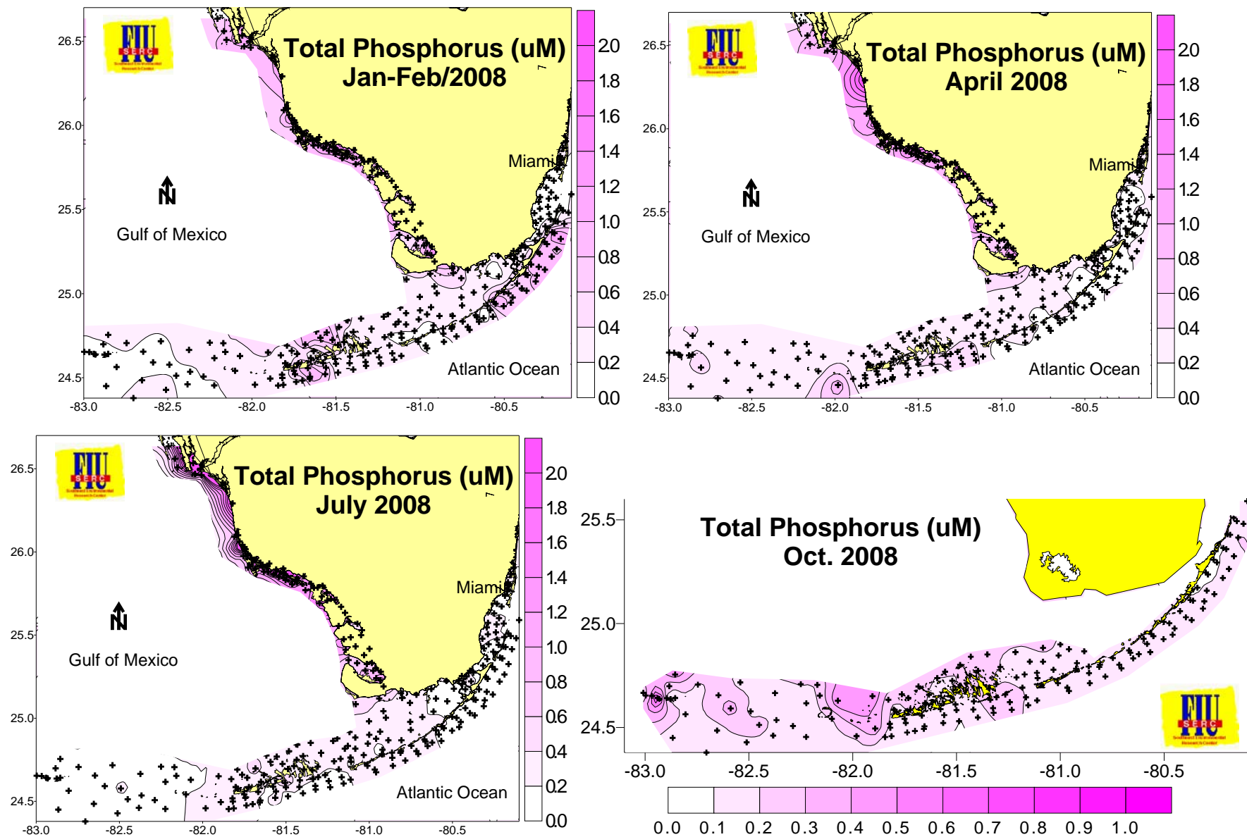
Figure 29. Distributions of total phosphorus across the region during 2008.
