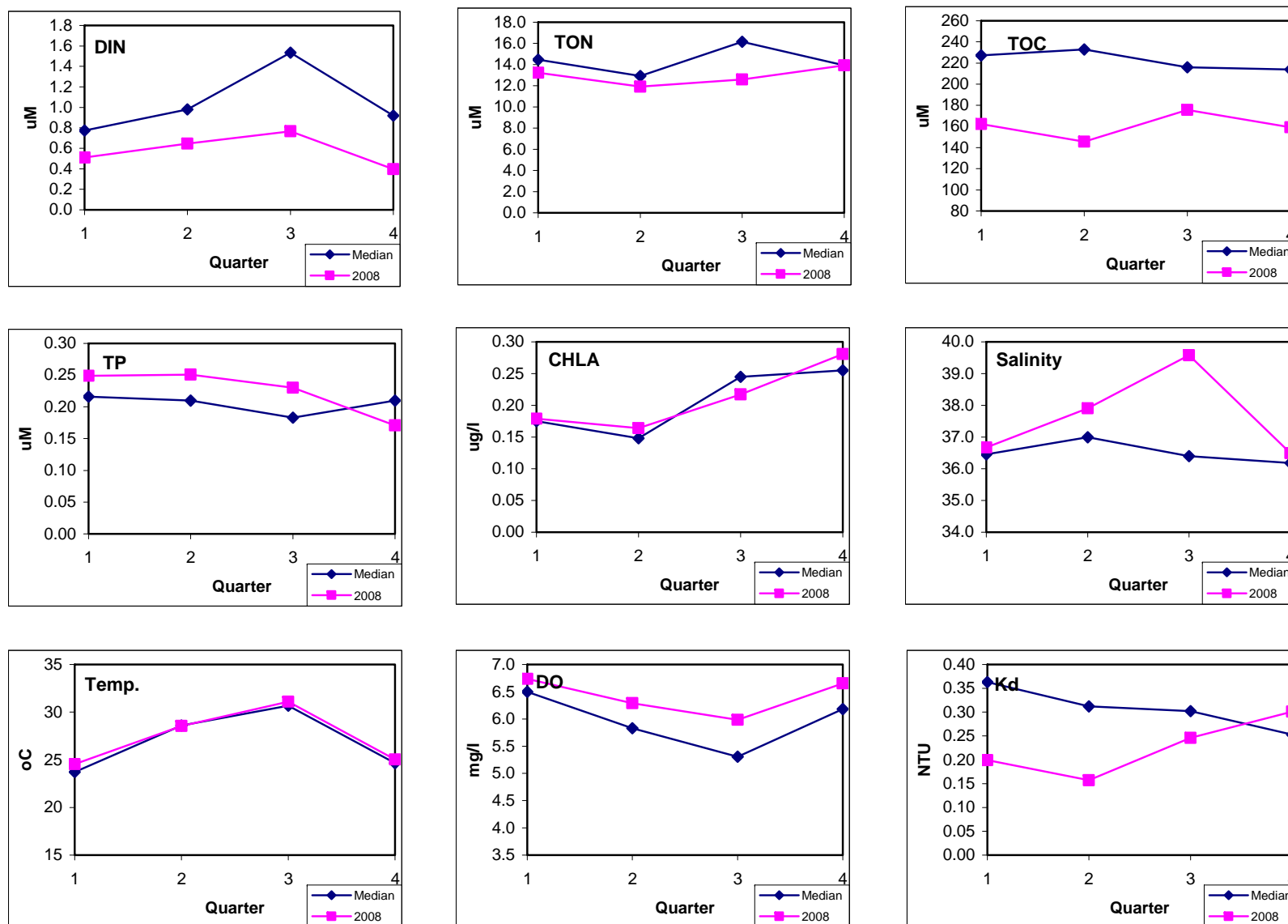
Figure 19. Comparison of long-term median with 2008 data.
