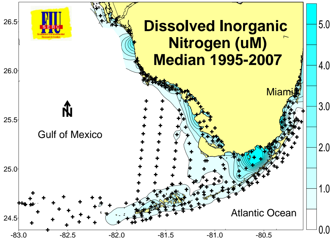
Figure 6. Median dissolved inorganic N (nitrate, nitrite, and ammonium) in the region.
