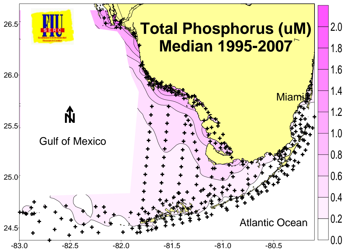
Figure 7. Distribution of median total phosphorus in the region.
