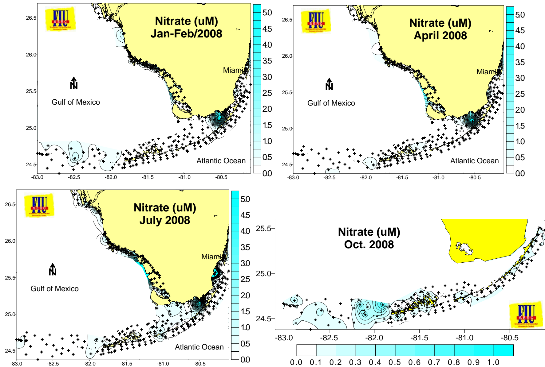
Figure 26. Nitrate distributions across the region during 2008.
