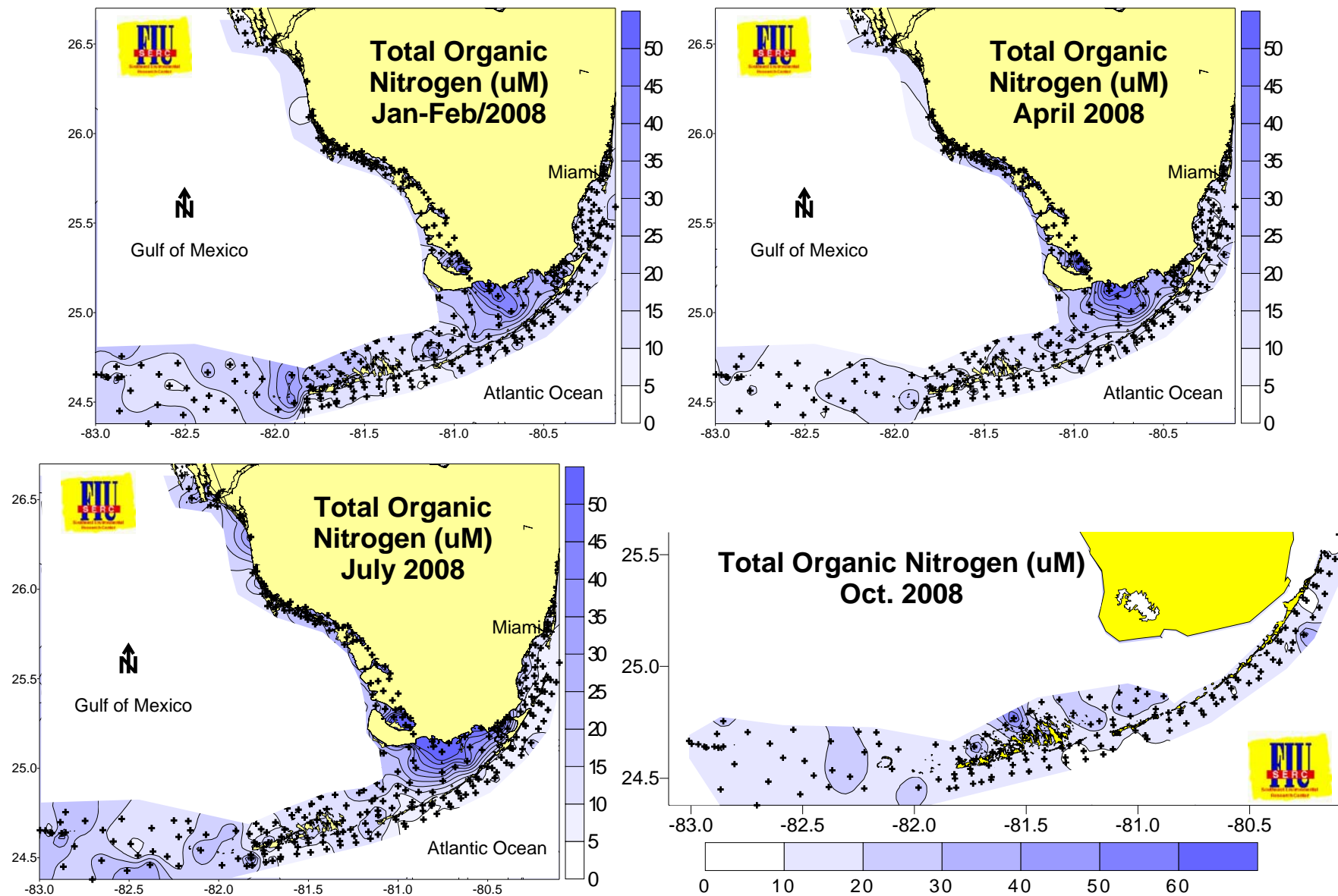
Figure 31. Distributions of total organic nitrogen across the region during 2008.
