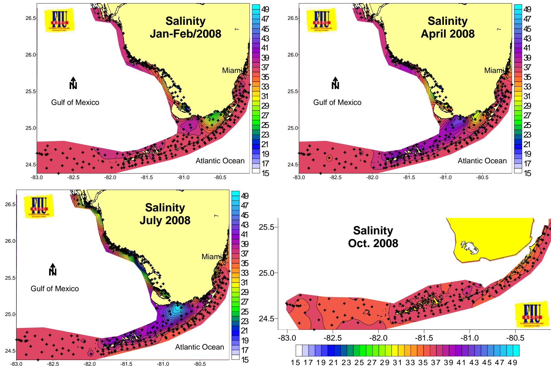
Figure 24. Salinity distributions across the region during 2008.
