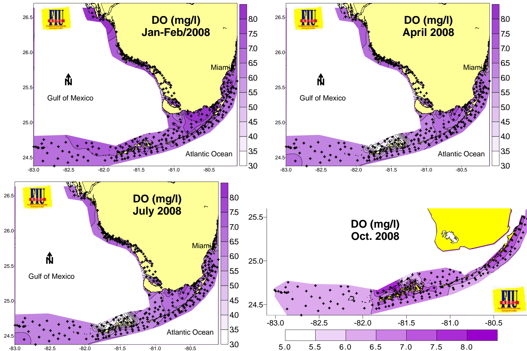
Figure 25. Dissolved oxygen distributions across the region during 2008.
