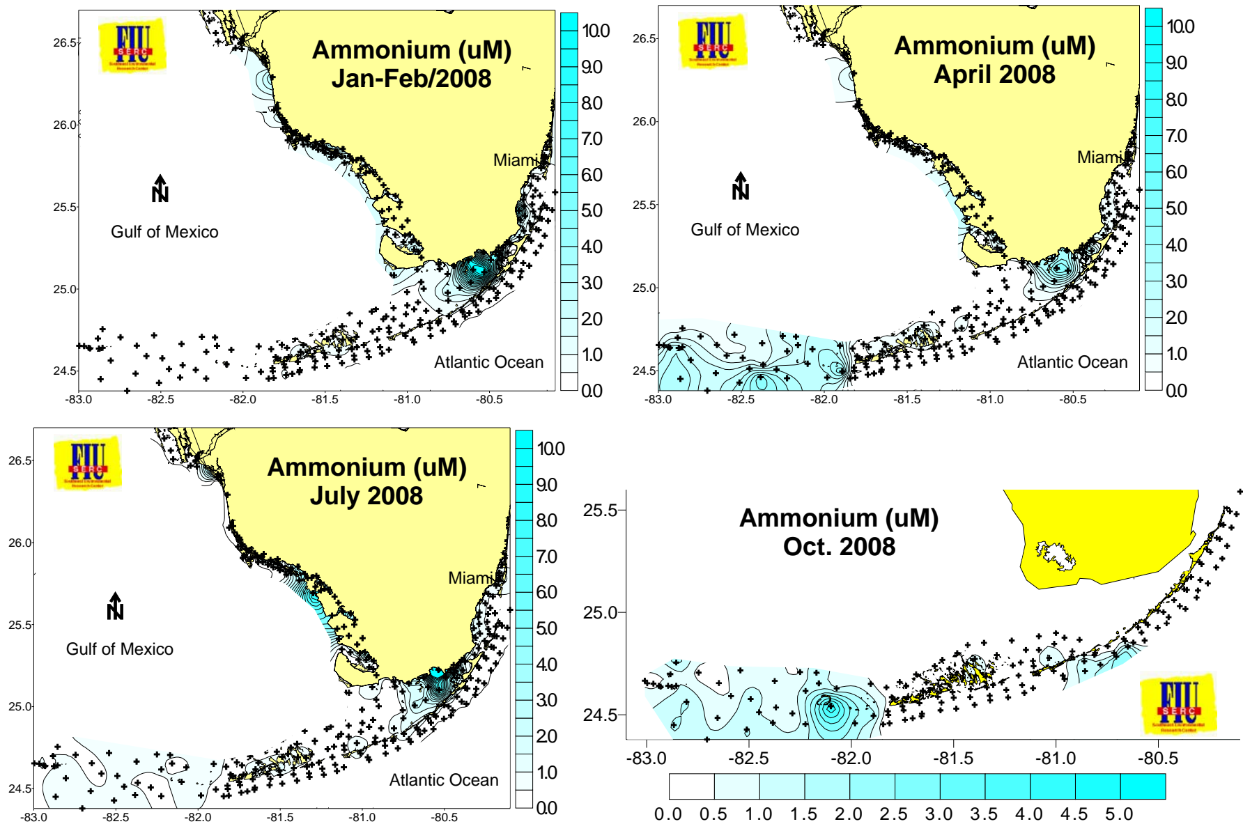
Figure 27. Ammonium distribution across the region during 2008.
