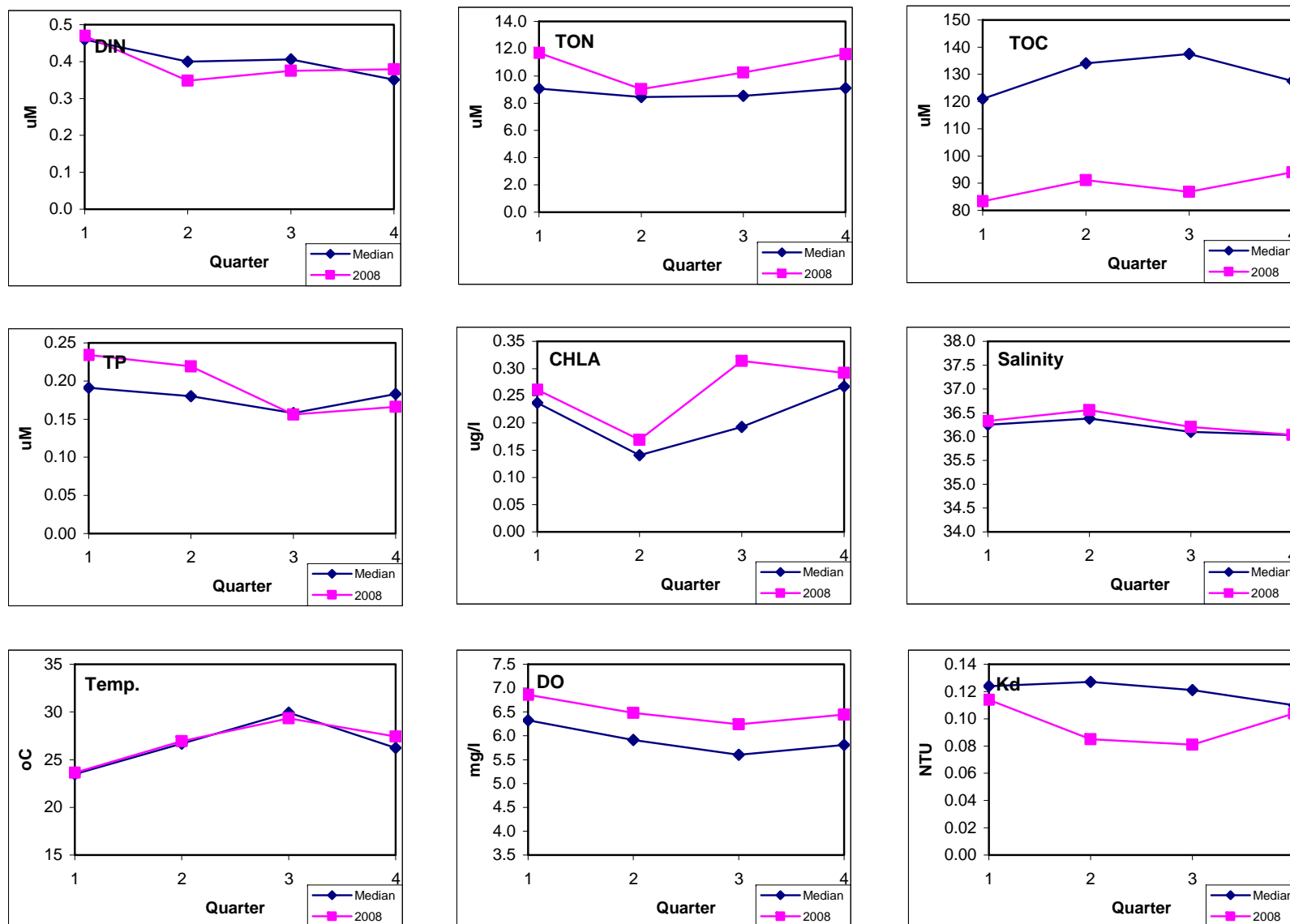
Figure 16. Comparison of long-term median with 2008 data.
