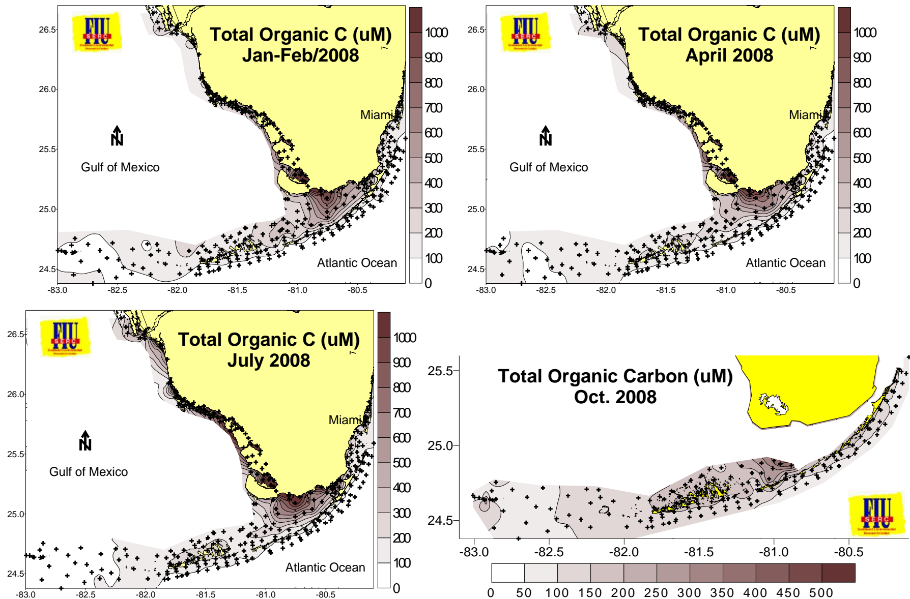
Figure 30. Distributions of total organic carbon across the region during 2008.
