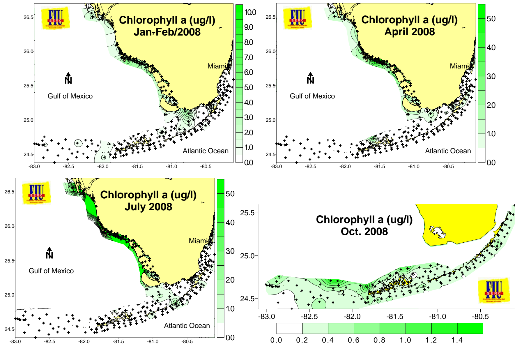
Figure 32. Distributions of chlorophyll a across the region during 2008.
