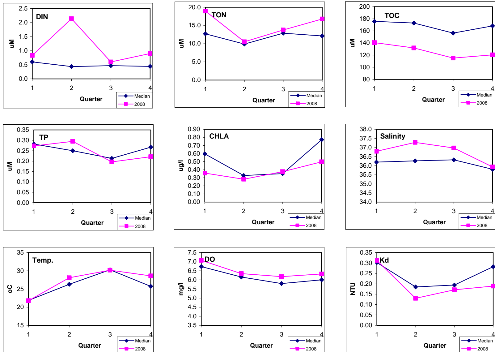
Figure 21. Comparison of long-term median with 2008 data.
