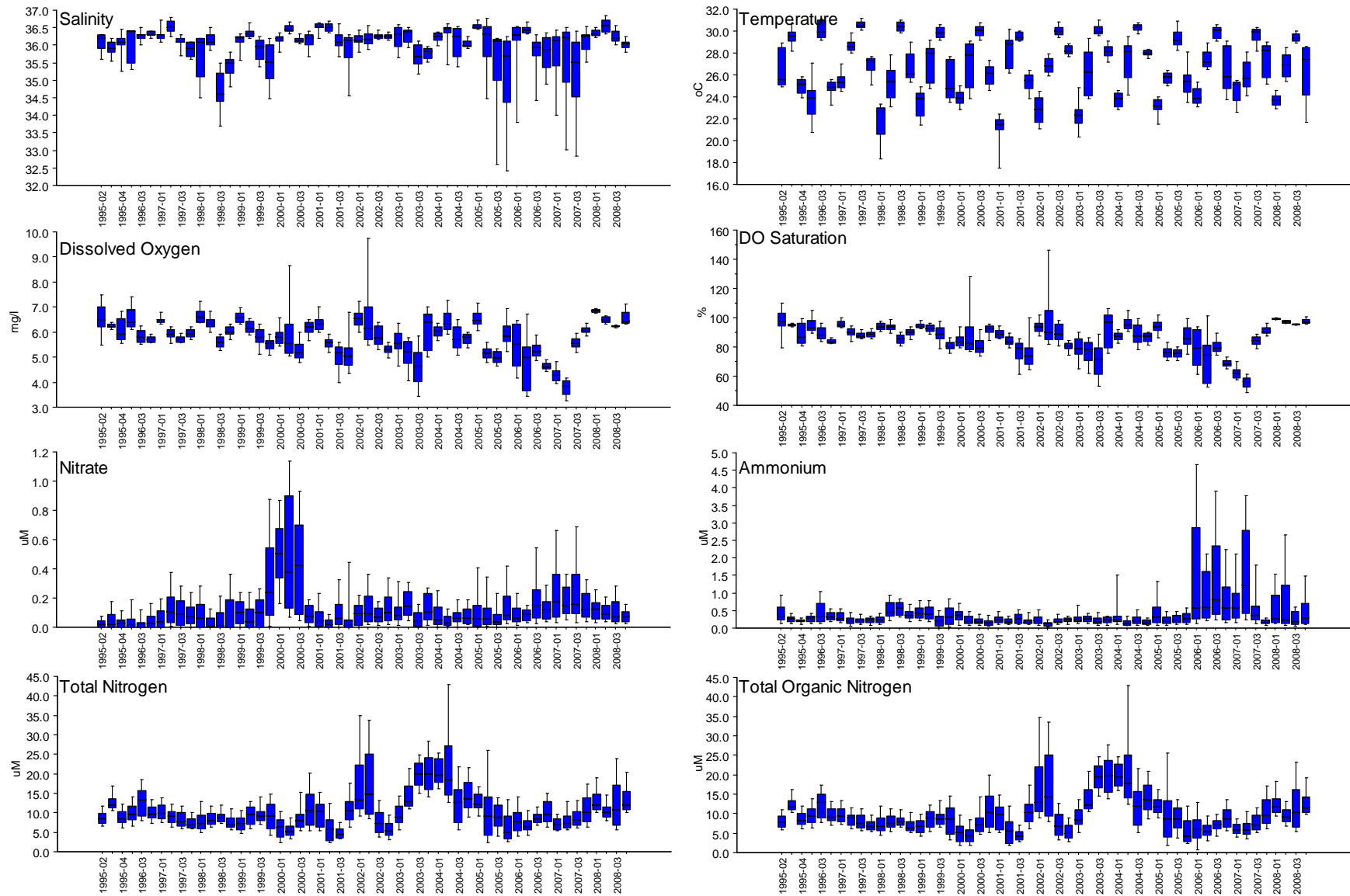
Figure 2. Selected water quality variables from the reef tract/Tortugas
