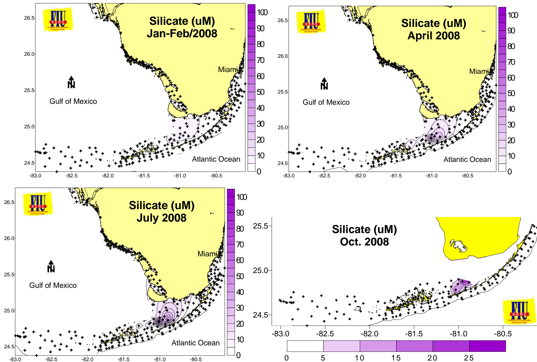
Figure 35. Distributions of silicate across the region during 2008.
