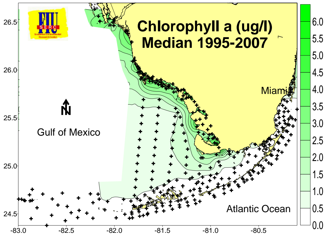
Figure 8. Median chlorophyll a in the region showing the similarity to TP distribution.
