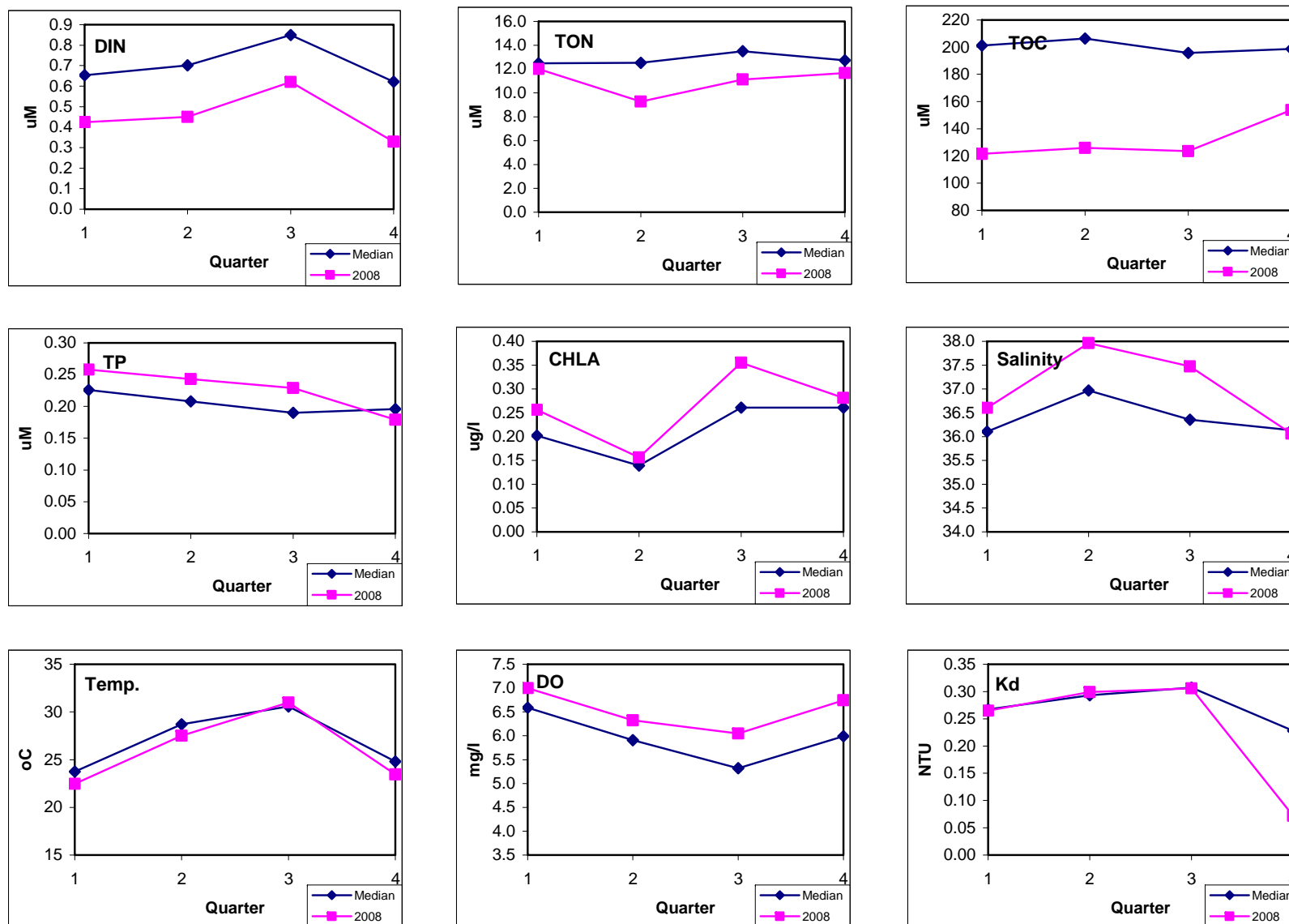
Figure 18. Comparison of long-term median with 2008 data.
