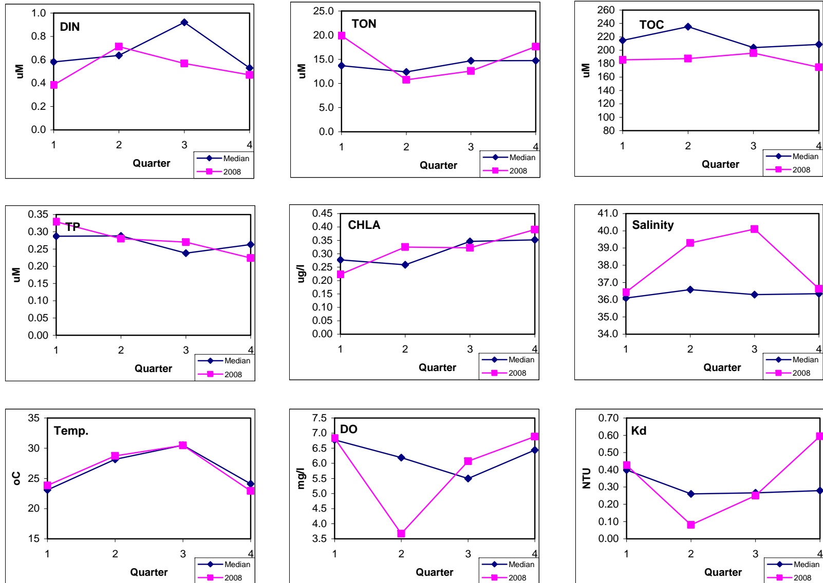
Figure 20. Comparison of long-term median with 2008 data.
