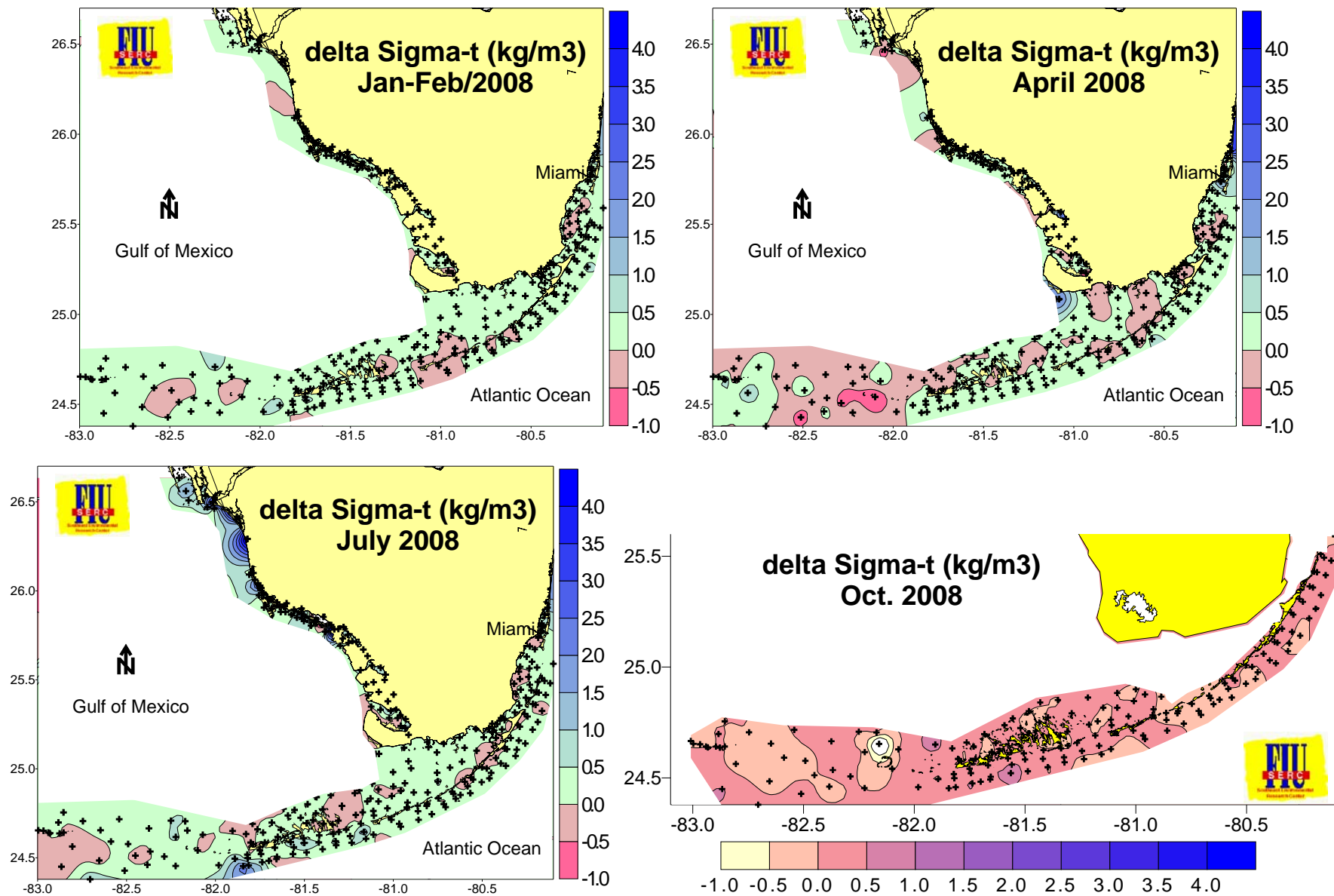
Figure 28. The distribution of water column stratification across the region during 2008.
