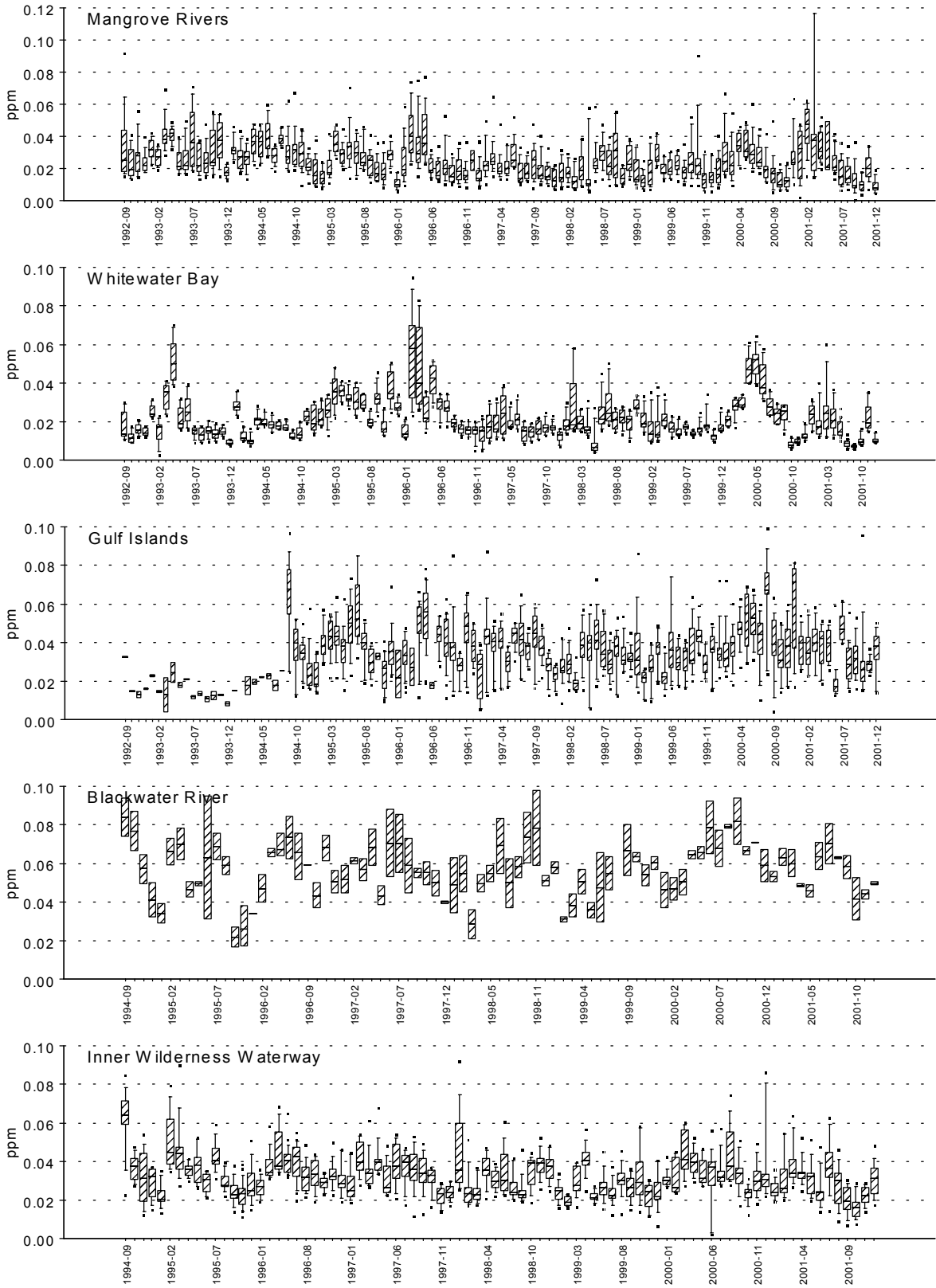
Figure 3.4. Monthly median and range of total phosphorus in the five WWB-TTI zones.
