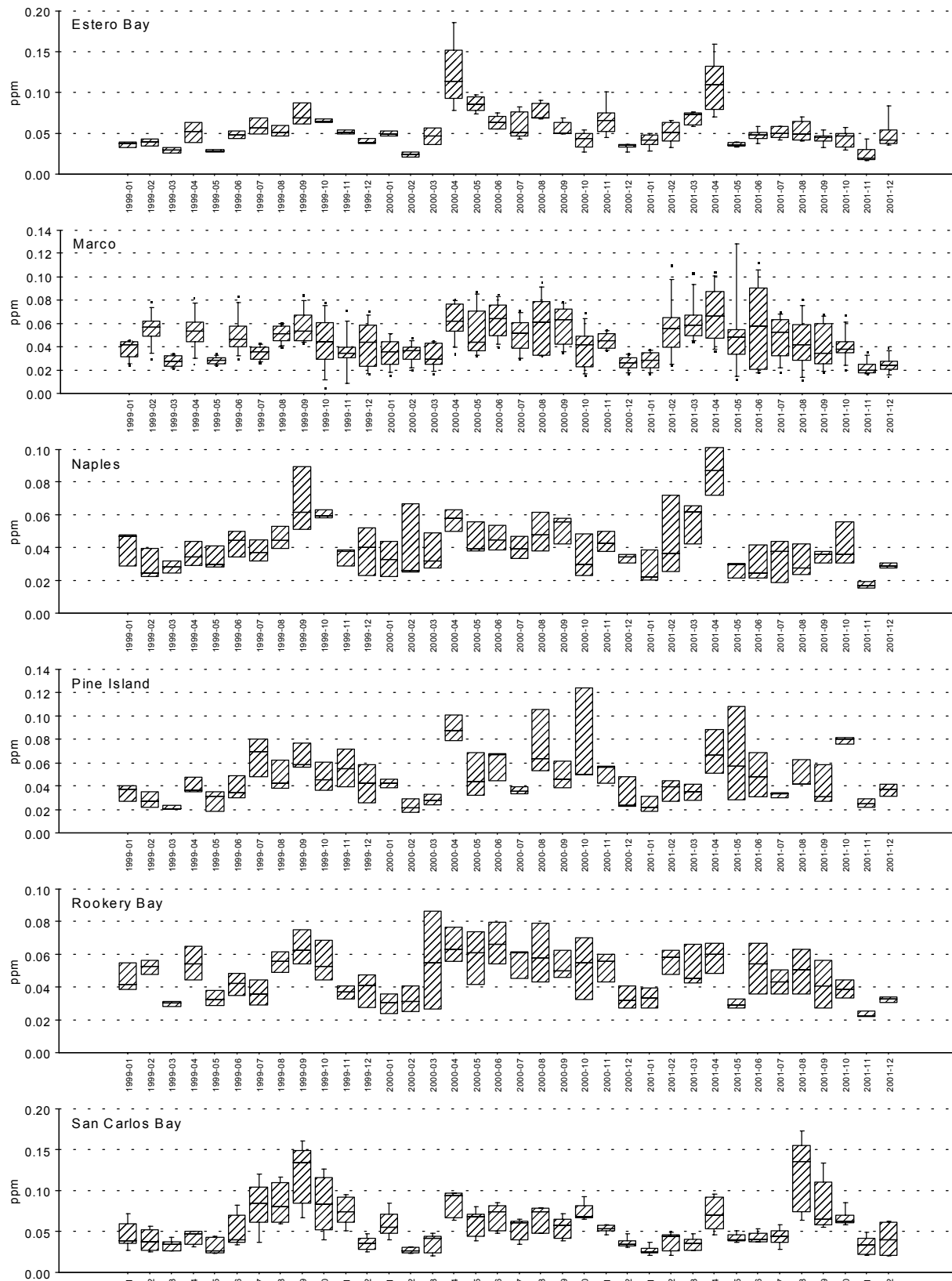
Figure 6.4. Monthly median and range of total phosphorus in the Cape Romano-PIS area.
