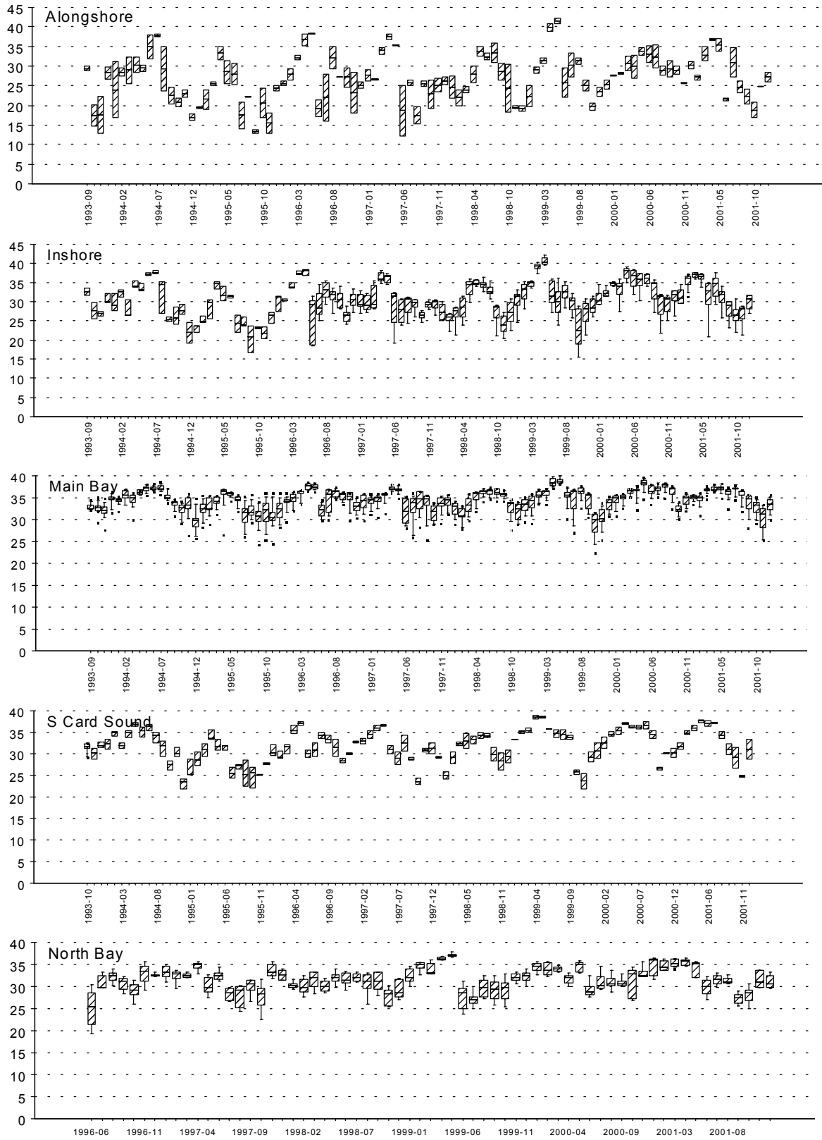
Figure 4.2. Monthly median and range of salinity in the five Biscayne Bay zones.
